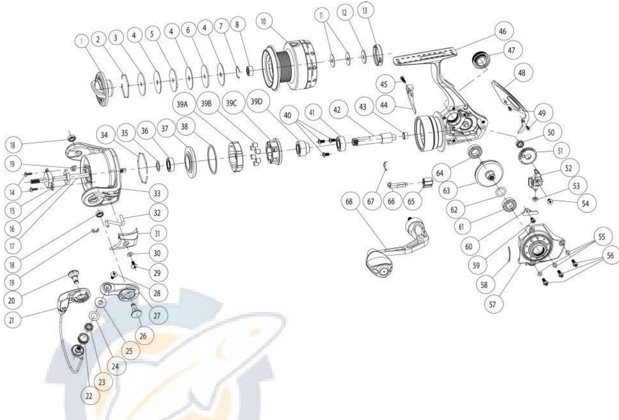
Quantum Tour Edition TE30PTIB Spinning Reel Part List
